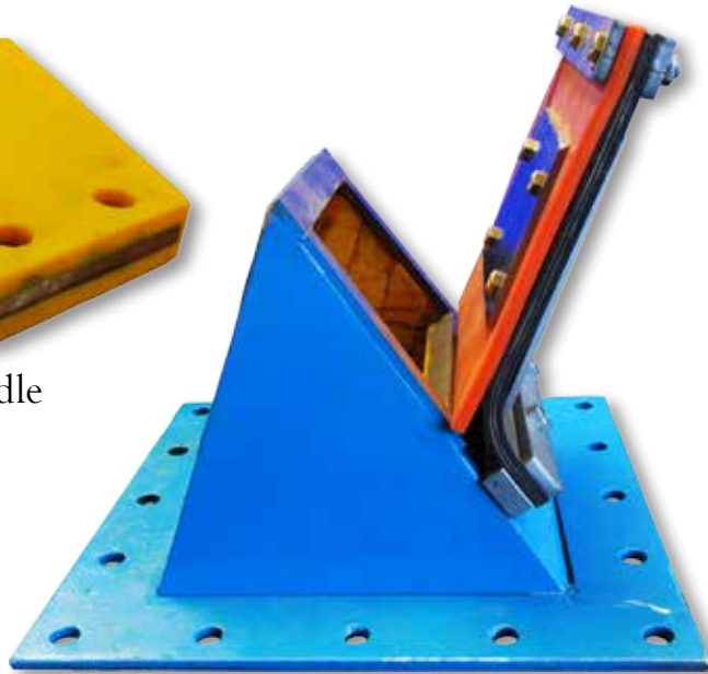
Urethane Sheet To Absorb Vibration On Chute Door
