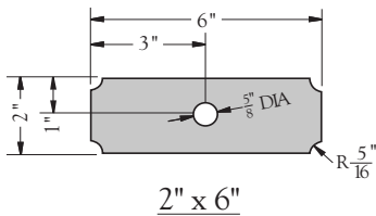
WearPads™ used to patch worn area.
