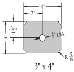
WearPads™ used to patch worn area.
